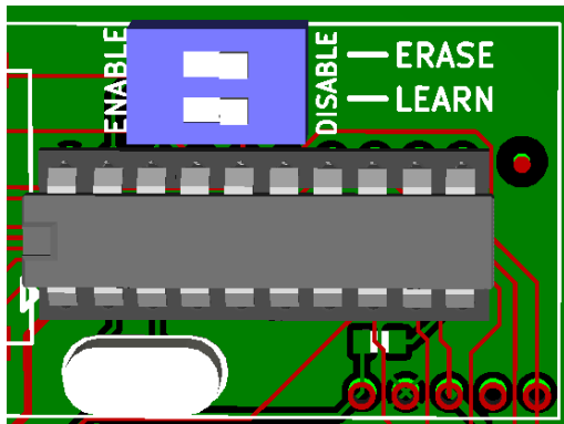
Figure 3 Learn/Erase Function
