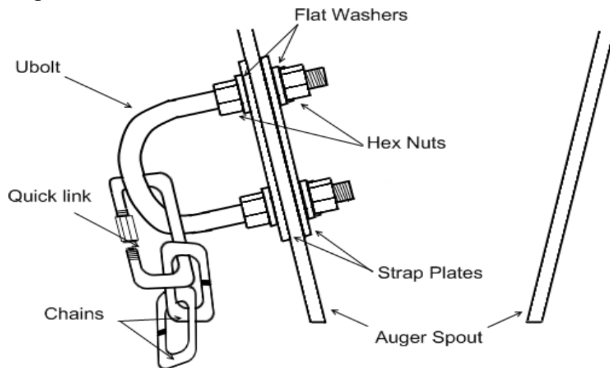
Figure 2 U-Bolt Instructions
